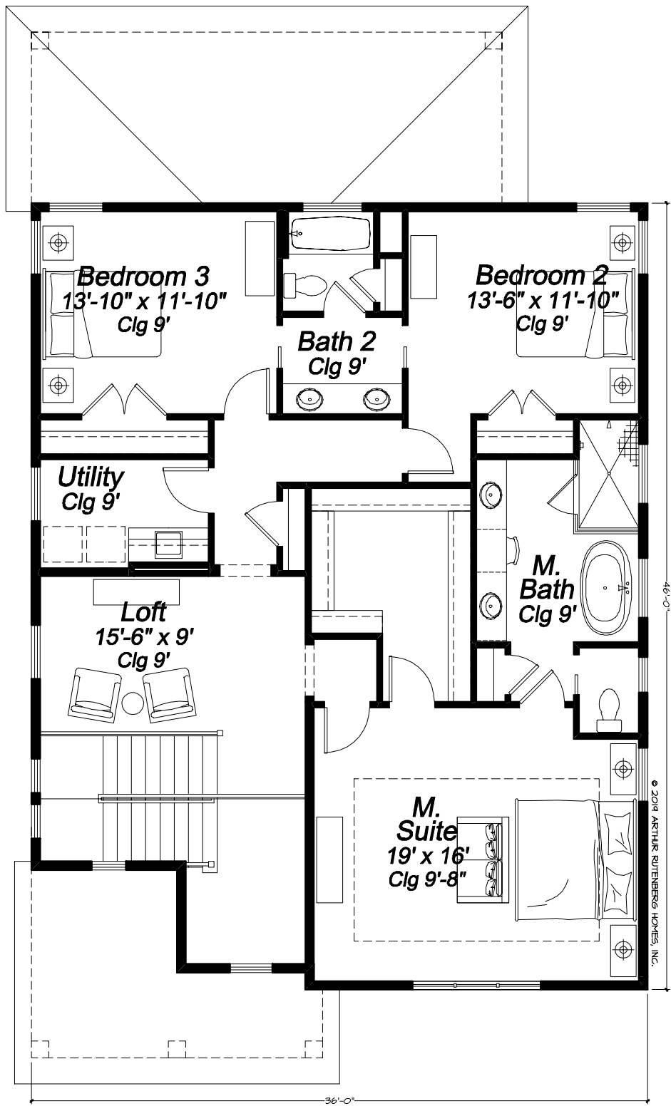
1709F Seville 2nd Floor Plan
